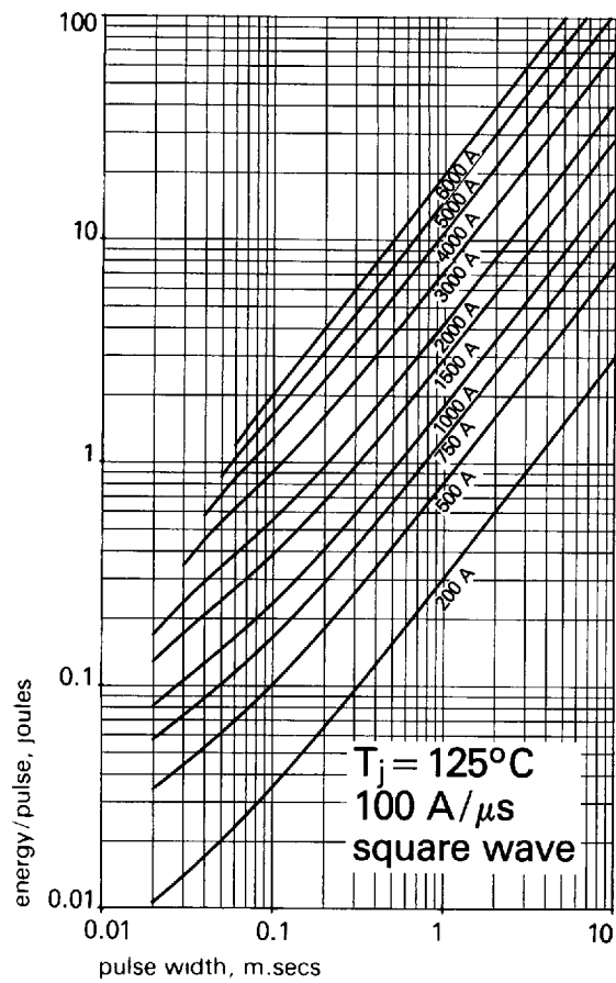
Figure 6 Energy/pulse v. pulse width
