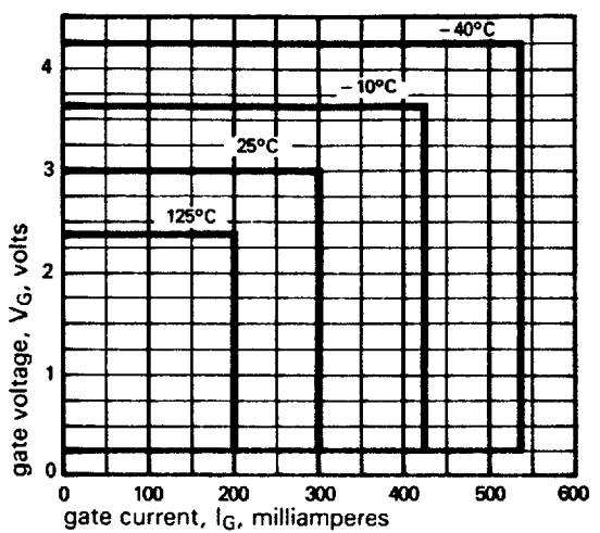
Figure 15 Gate triggering characteristics Trigger points of all thyristors lie within the areas shown
